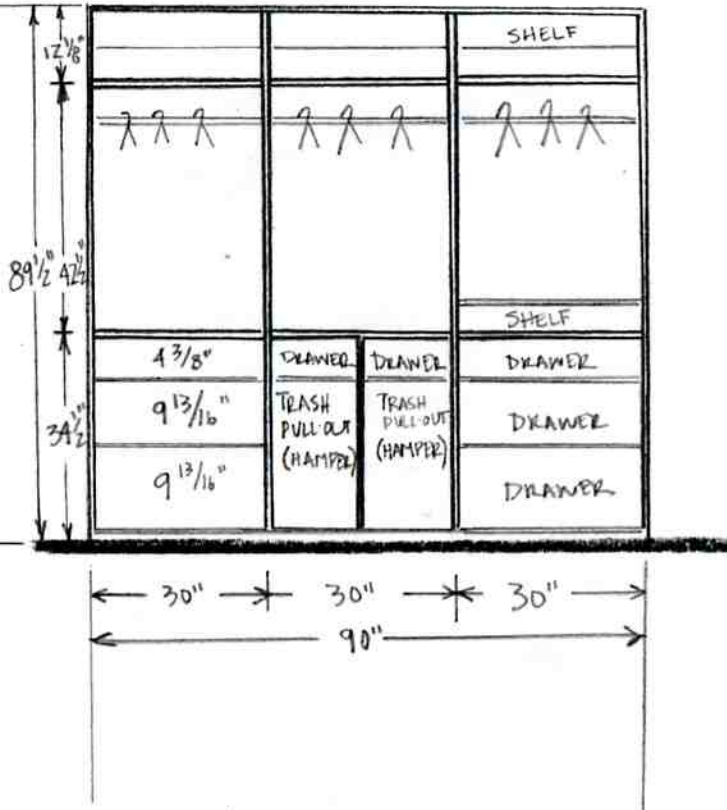
SECTION
